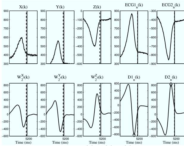
(b) ECG in orthogonal leads ( X(k) , Y(k) , Z(k) ), the correspondent WT signals ( W_{22}^X(k) , W_{22}^Y(k) , W_{22}^Z(k) ) and the new derived signals D1_n(k) and Dg_n(k) following the directions of vectors \mathbf{U1}_n and \mathbf{Ug}_n ( k \in t1_n ). Vertical dashed line stands for the T end mark found in the respective lead; solid line stands for manual based reference mark.
